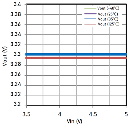
Line Regulation V_{OUT} vs. V_{IN} C_{OUT} = C_{IN} = 1 \mu F, I_{OUT} = 200 \text{ mA}
