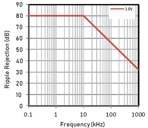
Ripple Rejection vs. Frequency I_{OUT} = 30 \text{ mA}, C_{OUT} = 1 \mu F
