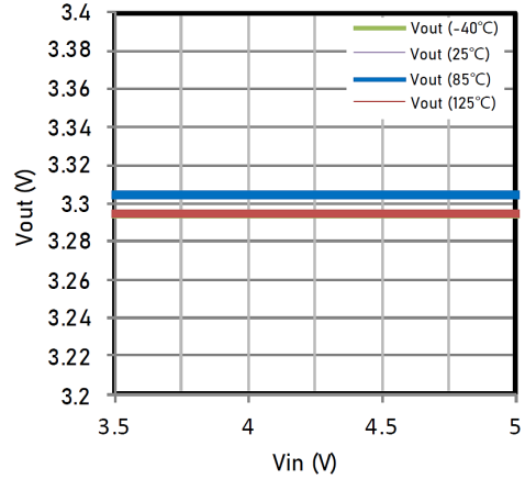
Line Regulation V_{OUT} vs. V_{IN} C_{OUT} = C_{IN} = 1 \mu F, I_{OUT} = 30 \text{ mA}
