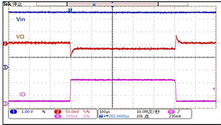
Load-Transient Response
