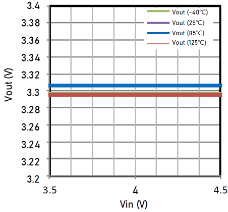
Line Regulation V_{OUT} vs. V_{IN} C_{OUT} = C_{IN} = 1 \mu F, I_{OUT} = 10 \text{ mA}
